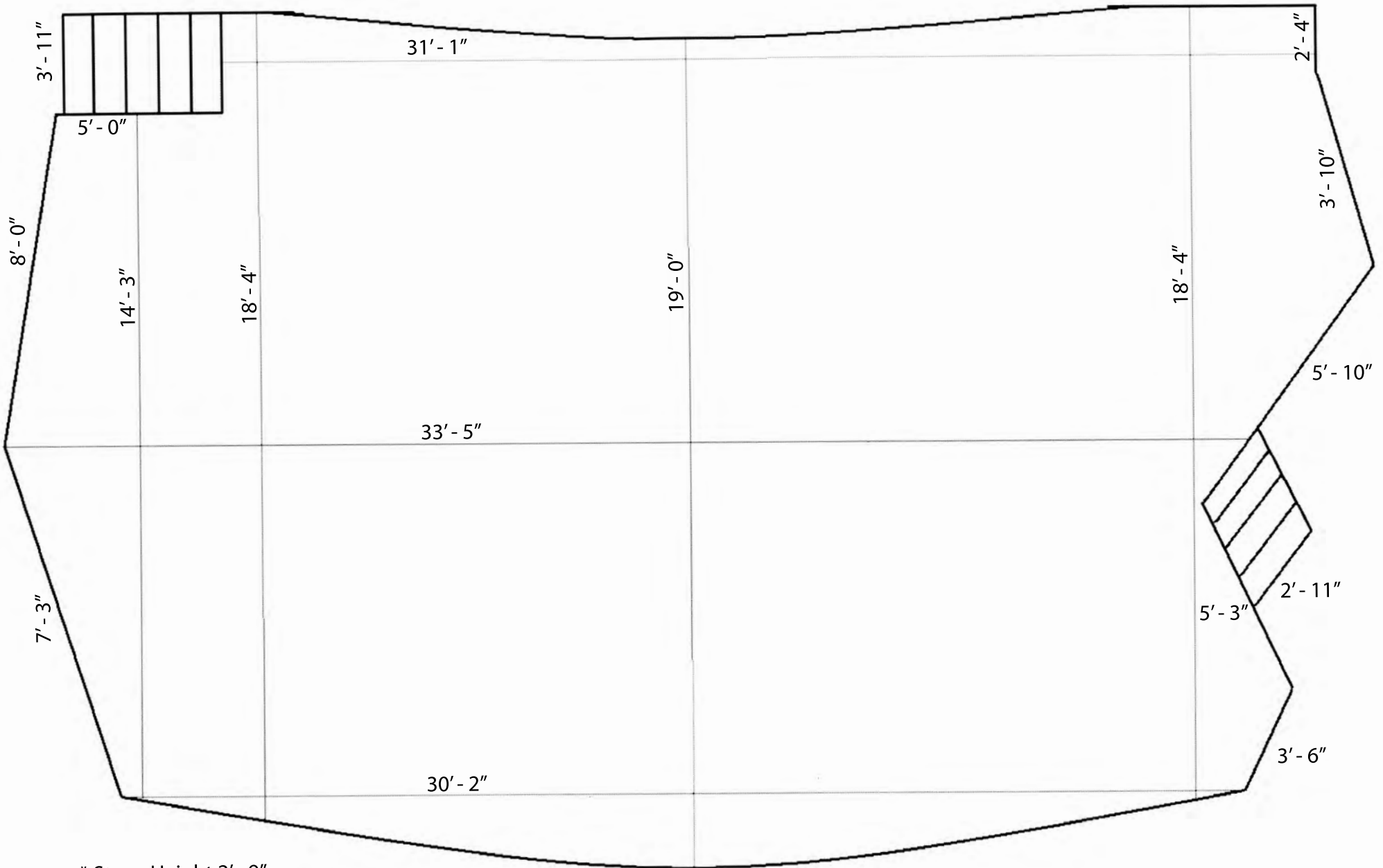
The State Theatre of Modesto, Inc. Stage Dimensions
